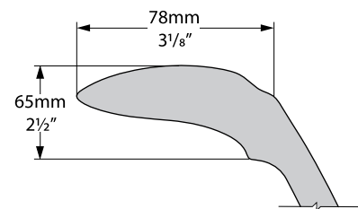
Rim detail
